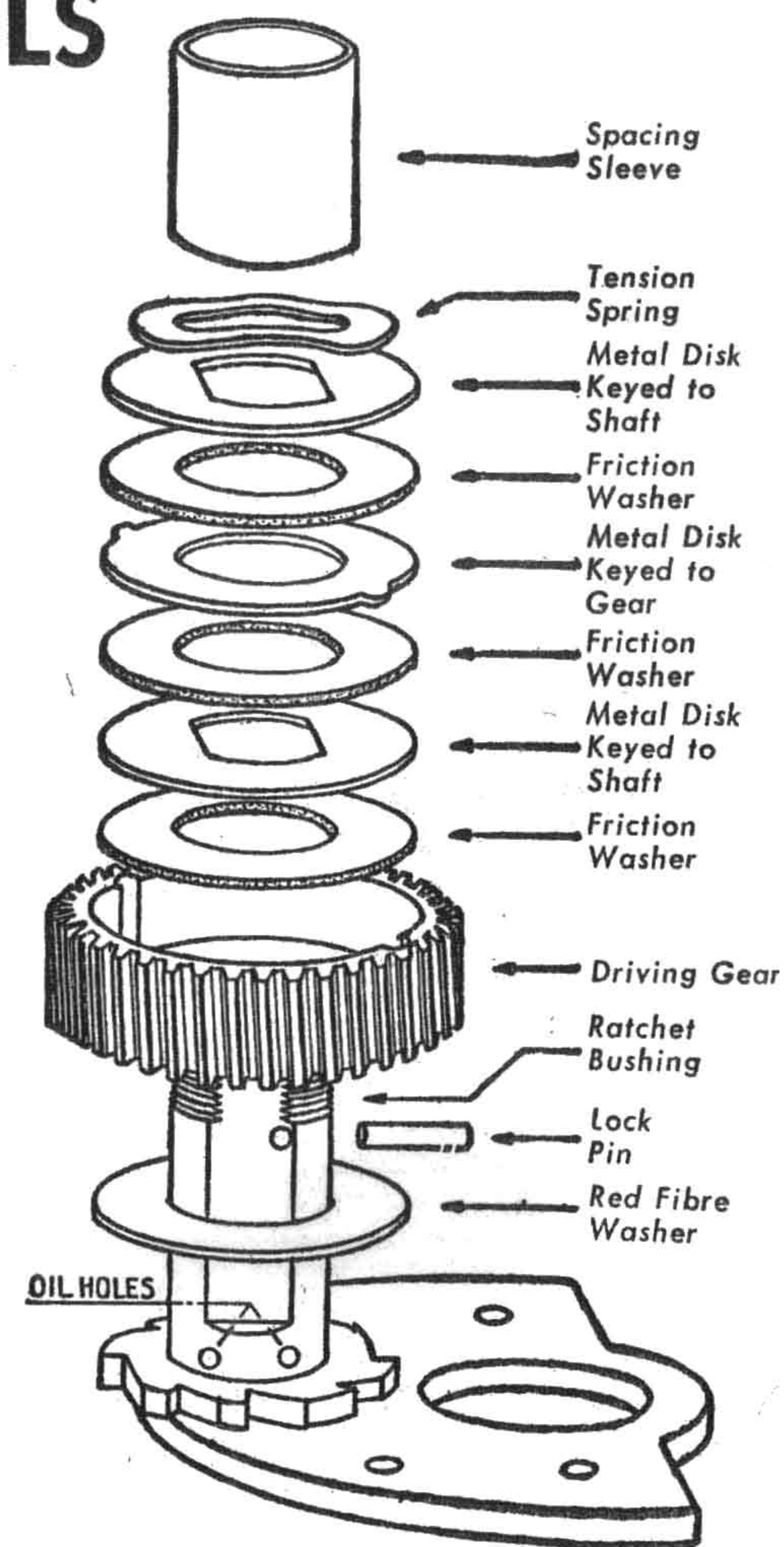
TYPICAL PENN DRAG ASSEMBLY
