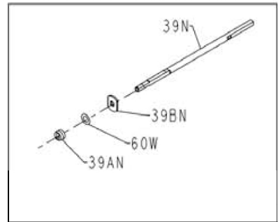
WASHER STYLE SPOOL SHAFT
