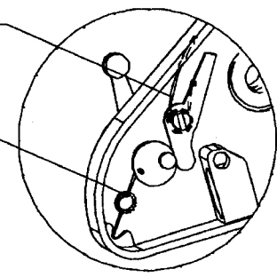
SPRING ASSEMBLY DETAIL
